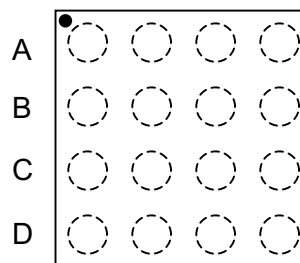
16-Ball CSBGA (4mm x 4mm)
